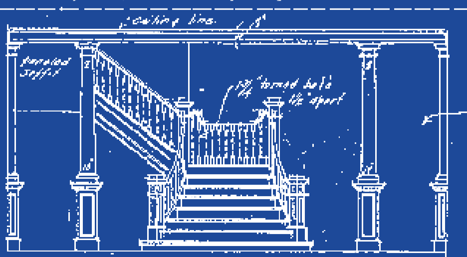
SCALE ELEVATION OF STAIR & GRILLE IN FRONT HALL
